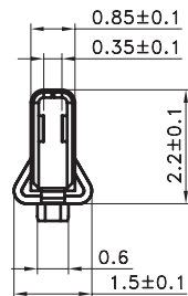
SEC.C-C
